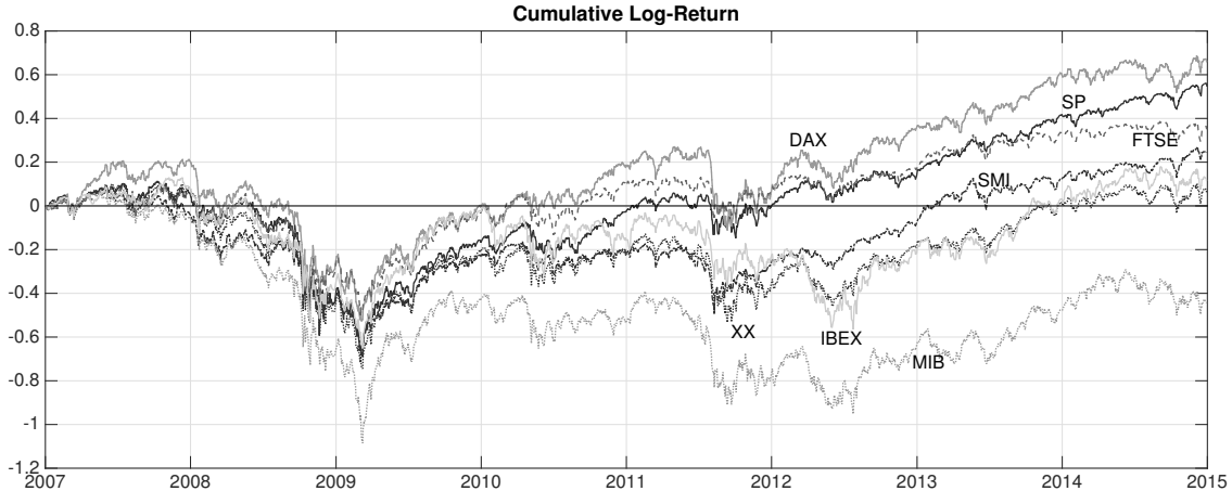
Figure 1: Country-specific cumulative equity-index cum dividend log-returns. The source of the data used in constructing the figure are detailed in Section 3.
